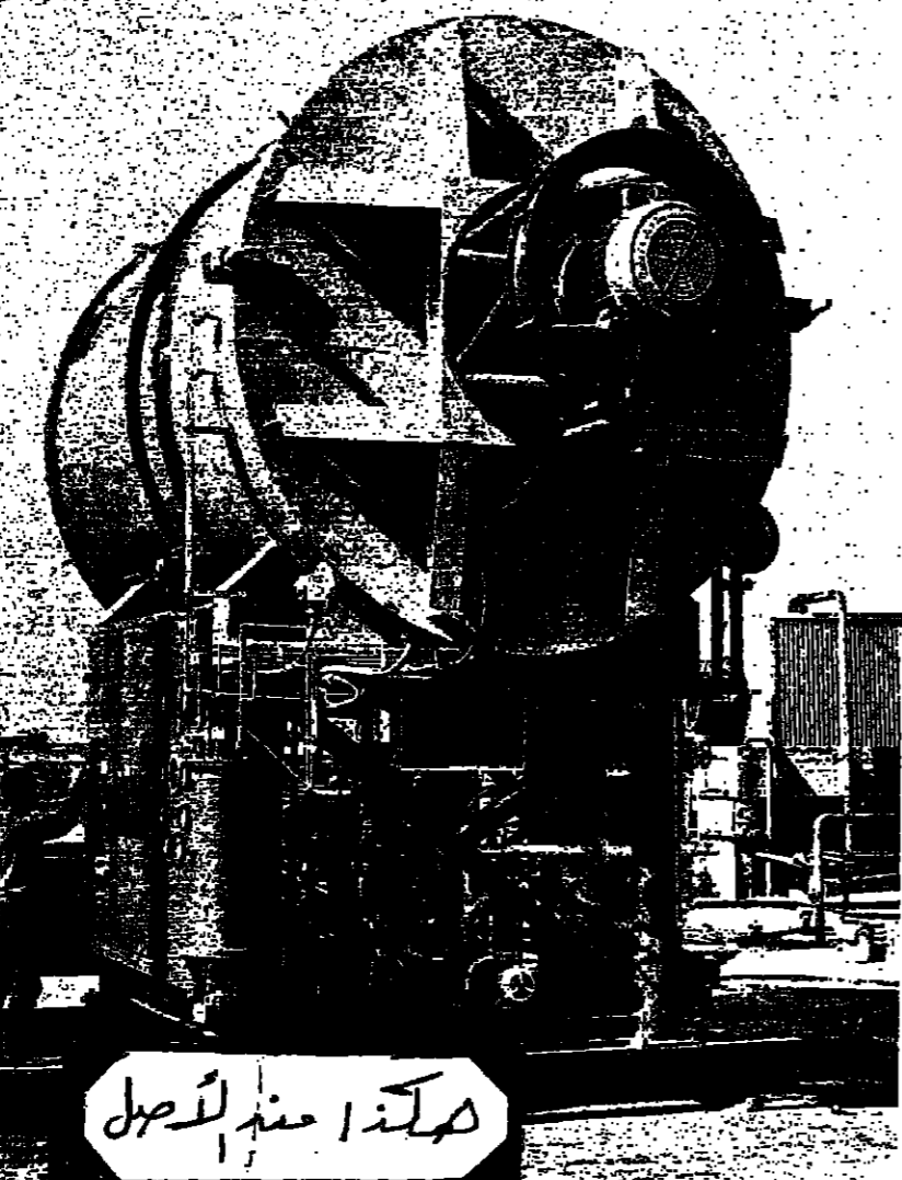
Israel occupies a leading place in research and development of desalination plants and a local company, Israel Desalination Engineering, supplies units to many parts of the world. Here a unit with a daily capacity of 100 cubic metres is tested before being loaded for export to Spain.
